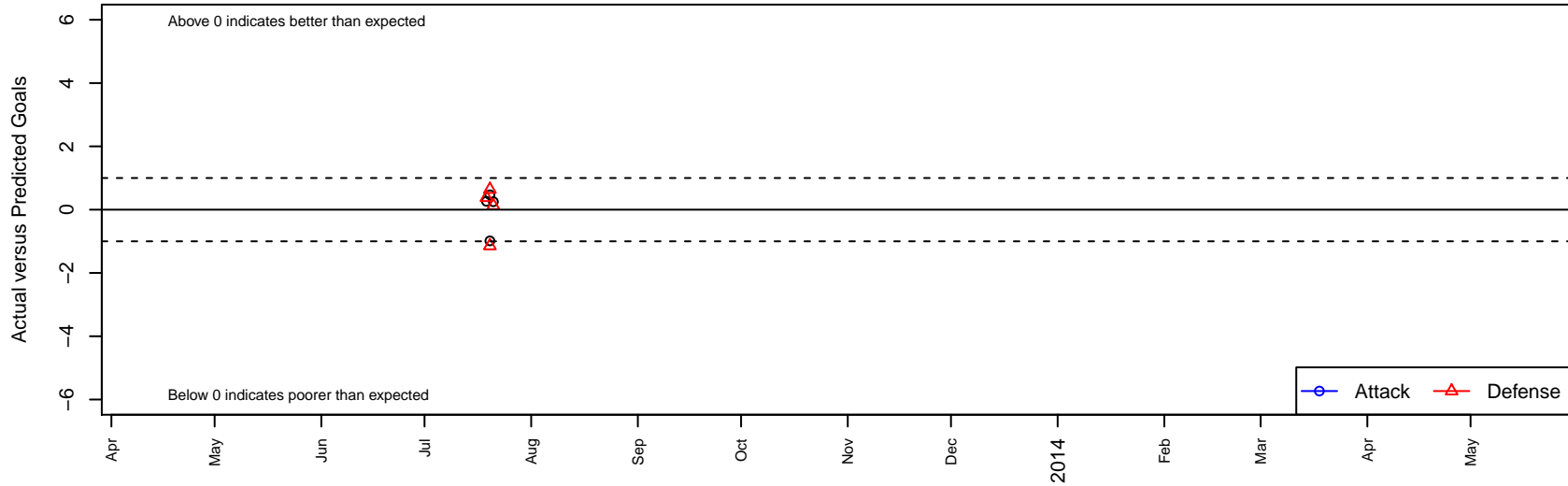
TCF -Unk B97 Dots are actual minus expected GF (blue circles) and GA (red triangles). Blue line is smoothed change in attack strength. Red is smoothed change in defense strength.
